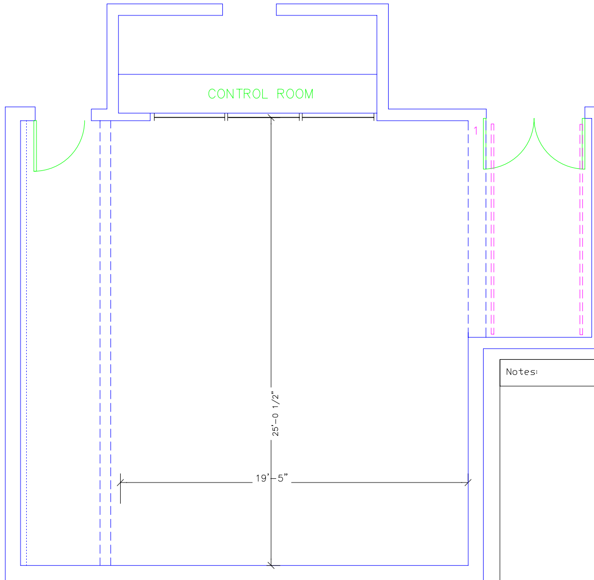
59E59 Theaters THEATER C Basic Groundplan
